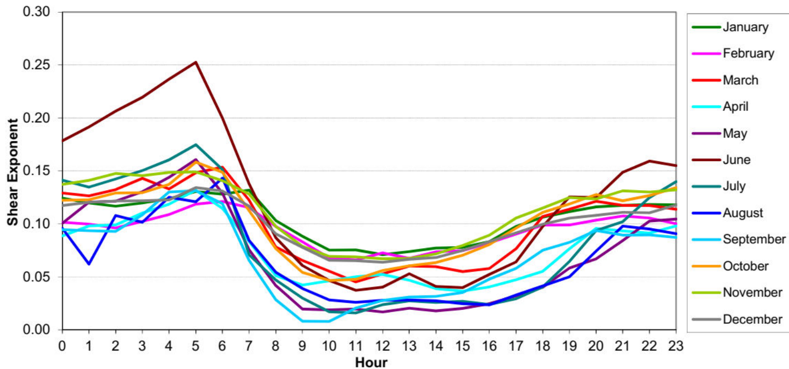
Figure 2-3. Monthly and Hourly Wind Shear at Changhua Met Tower
